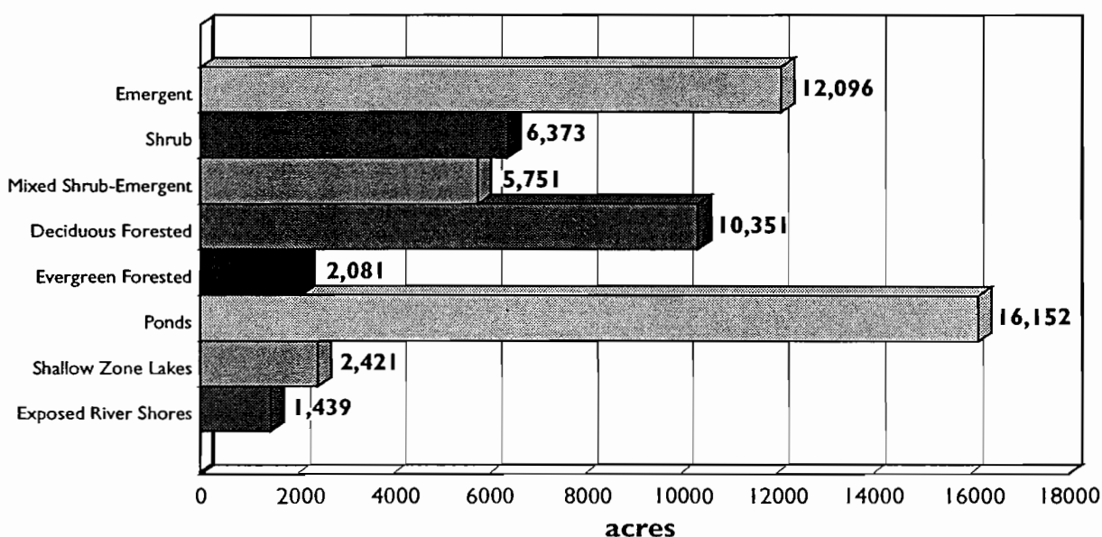
Figure 4-3. Extent of wetland types in West Virginia based on NWI mapping.
